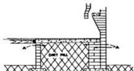
Chimney Base (Figure 4)
